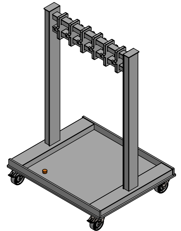
ISO VIEW HOOKS SPACED EVENLY
